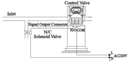
Figure 3-4 Wiring of Pressure Relief Port
