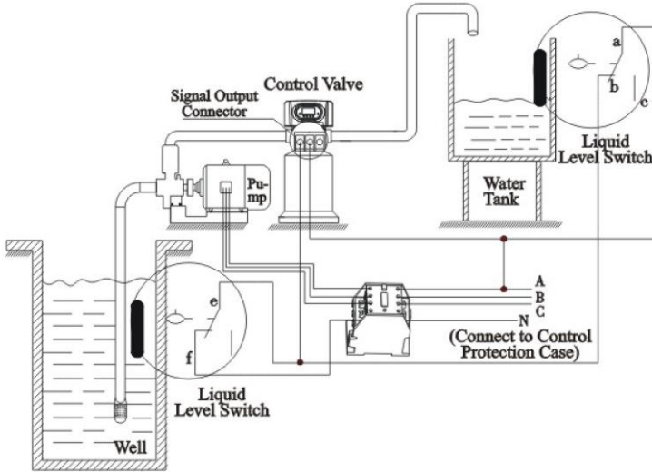
Figure 3-7 Wiring of Liquid Level Switch in Water Tank Controls 380V Inlet Pump
