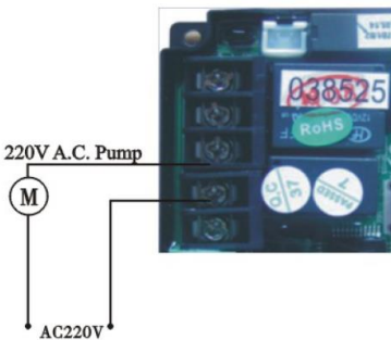
Figure 3-8 Wiring of Booster Pump on Inlet
